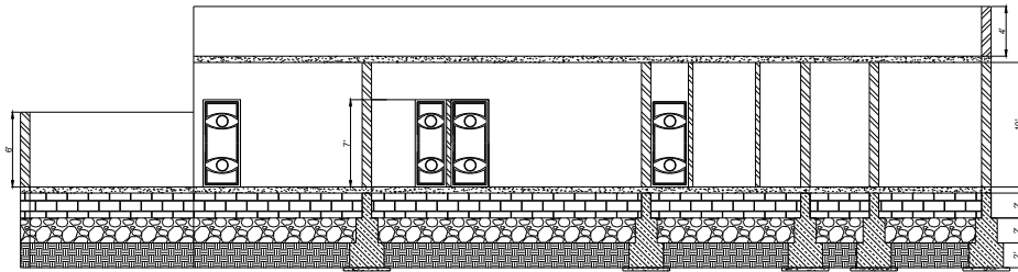
RIGHT SECTION
