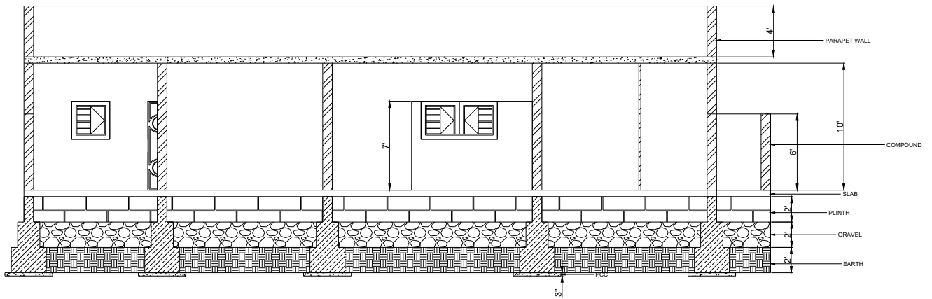
BOTTOM SECTION
