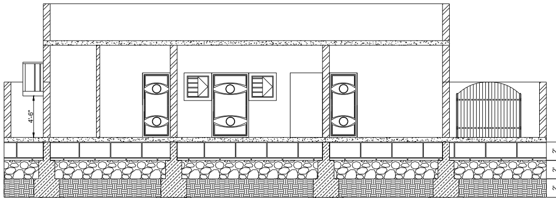
TOP SECTION
